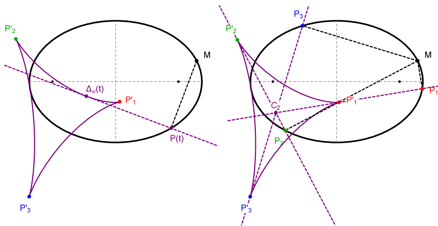
Figure 2: Left: The Negative Pedal Curve (NPC, purple) of \mathcal{E} with respect to a boundary point M is a 3-cusped (labeled P_i^j ) asymmetric curve (called here “Steiner’s Hat”), whose area is invariant over M , and whose asymmetric shape is affinely related to the Steiner Curve [12]. \Delta_u(t) is the instantaneous tangency point to the Hat. Right: The tangents at the cusps points P_i^j concur at C_2 , the Hat’s center of area, furthermore, P_i, P_i^j, C_2 are collinear. Video: [10, PL#01]
