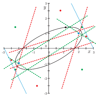
Figure 11: Three sets of foci and directrices
